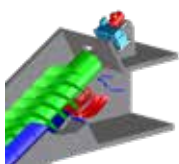
Hydropower screw pump for waterway Wilhelminakanaal, Tilburg, the Netherlands
